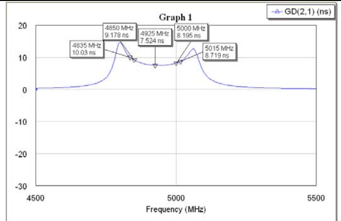
Group Delay
