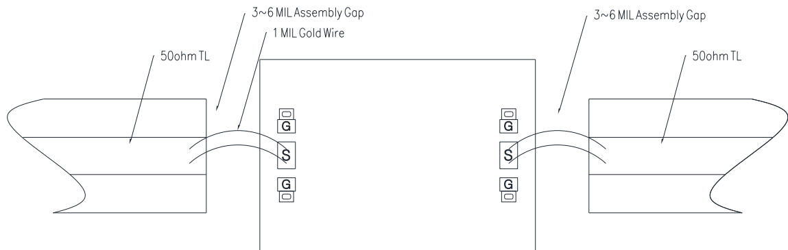
Assembly Diagram
