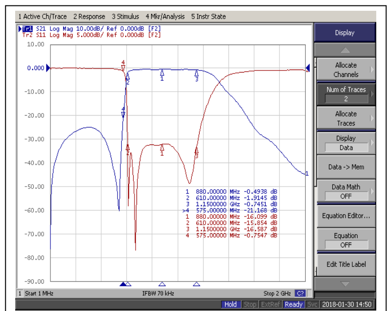
[ TEST CURVE ]
