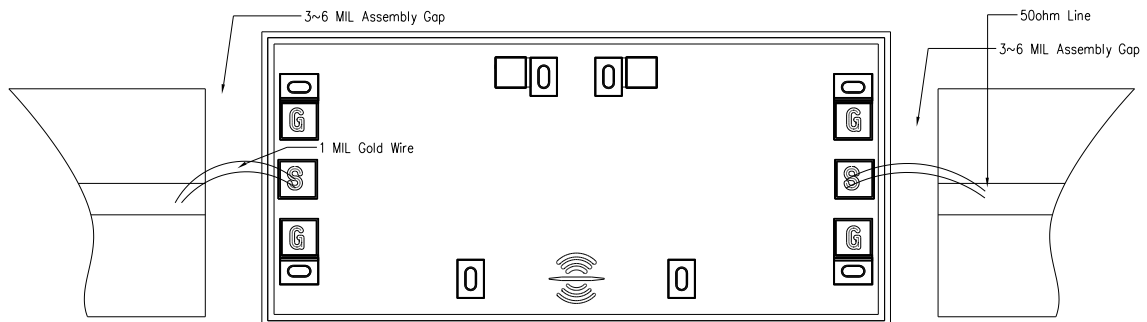
Assembly Diagram
