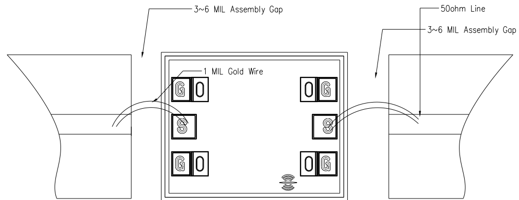
Assembly Diagram
