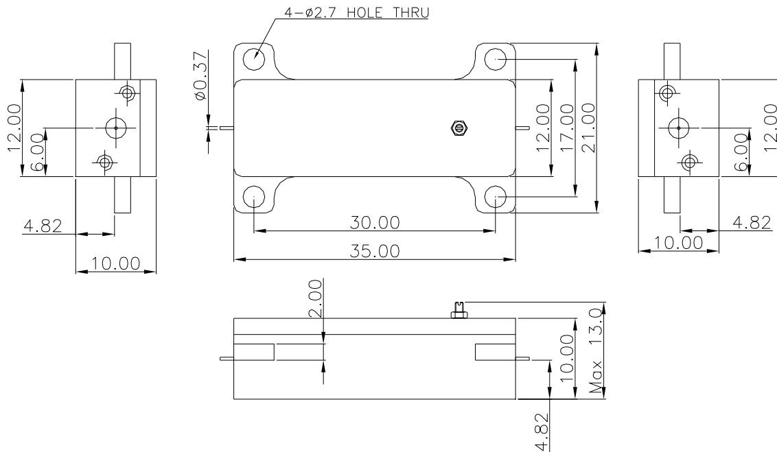
[ Mechanical 2D Drawing ]
